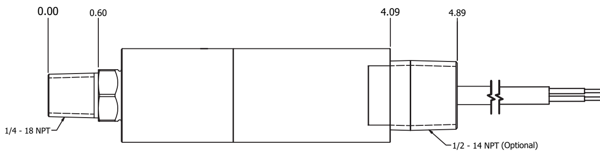
Typical P400 with 1/4 - 18 NPT and jacketed leads (other configurations available)
